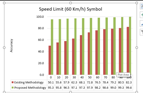
Fig. 8: Accuracy analysis of speed limit (60km/hr) traffic symbol
