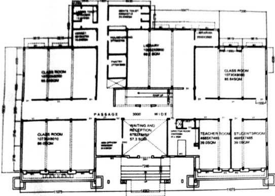
BLOCK-1 GROUND FLOOR PLAN
