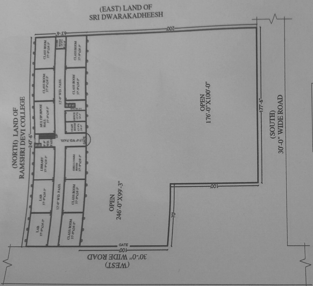
EXIST. G.F. PLAN
