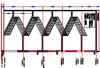
SECTION X-X' SCALE-1:100
