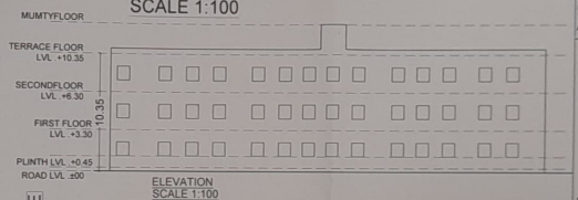
ELEVATION SCALE 1:100
