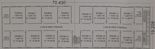
SECOND FLOOR PLAN SCALE 1:100
