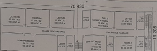
FIRST FLOOR PLAN SCALE 1:100
