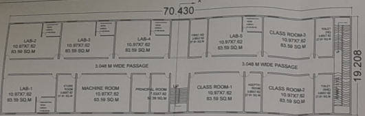
GROUND FLOOR PLAN SCALE 1:100
