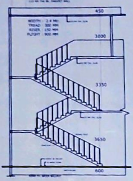
SECTION AT A-B
