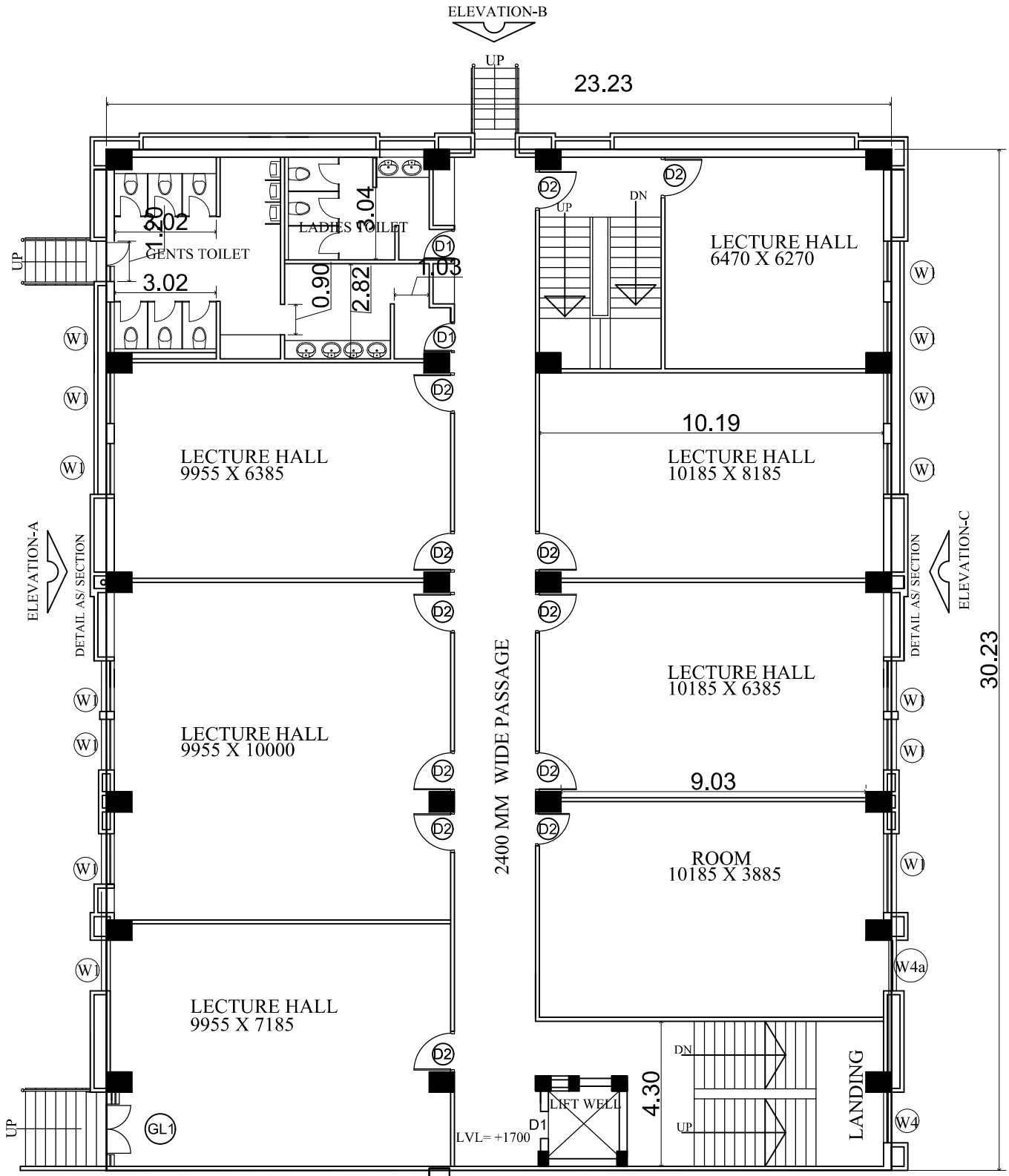
GROUND FLOOR PLAN 702.242 SQ.M
