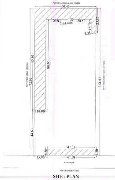
TERRACE PLAN (SCALE - 1:200)
