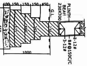
DETAILS OF PLINTH BEAM
