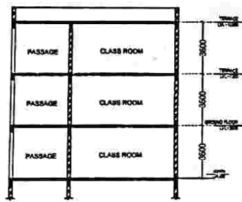
SECTION A-A' SCALE - 1:100
