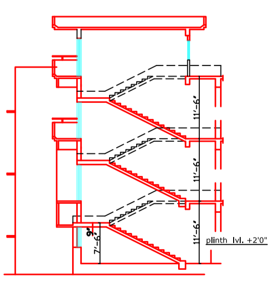
SECTION AT A-A
