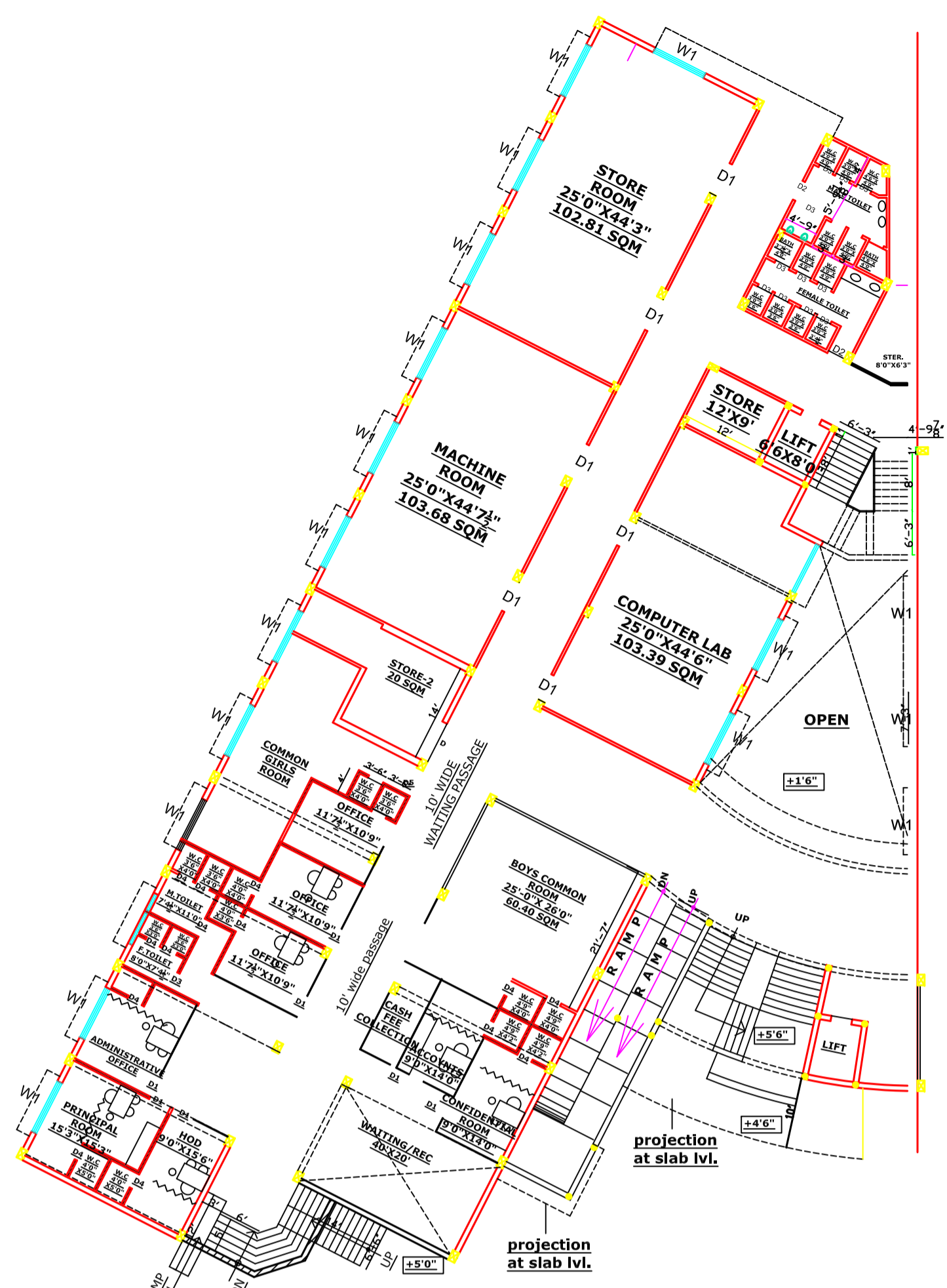
GROUND FLOOR
