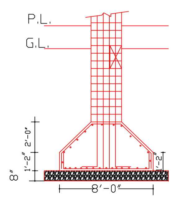
COLUMN FOUNDATION
