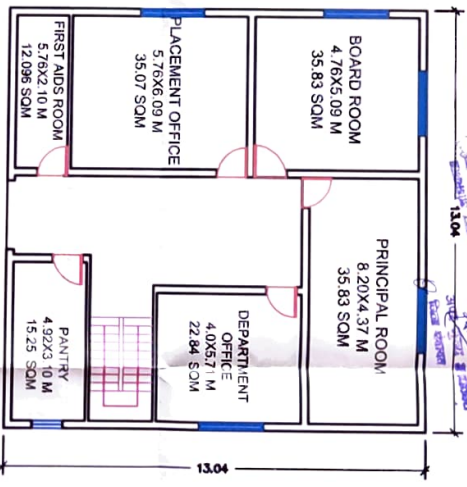
ADMINISTRATIVE AREA GROUND FLOOR PLAN SCALE-1:100
