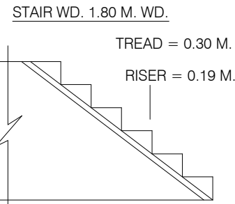
STAIR DETAIL
