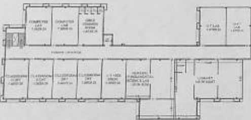
EXISTING THIRD FLOOR PLAN SCALE 1:100
