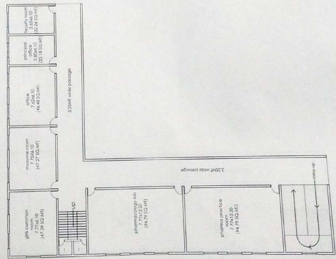
BLOCK-A GROUND FLOOR PLAN
