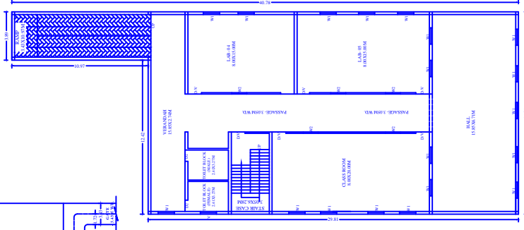
SECOND FLOOR PLAN SCALE = 1:100
