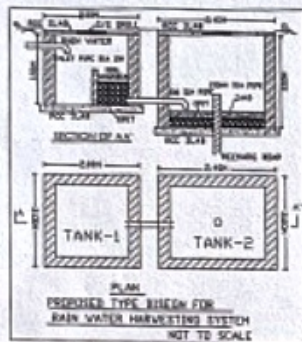
PROPOSED TYPE DESIGN FOR RAIN WATER HARVESTING SYSTEM NOT TO SCALE
