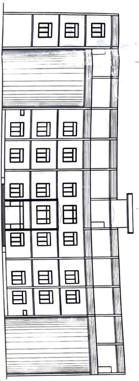
IRON ELEVATION
