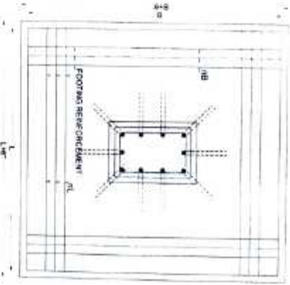
FOUNDATION DETAIL PLAN
