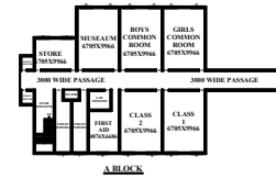
EXIST. GROUND FLOOR PLAN SCALE: 1/50
