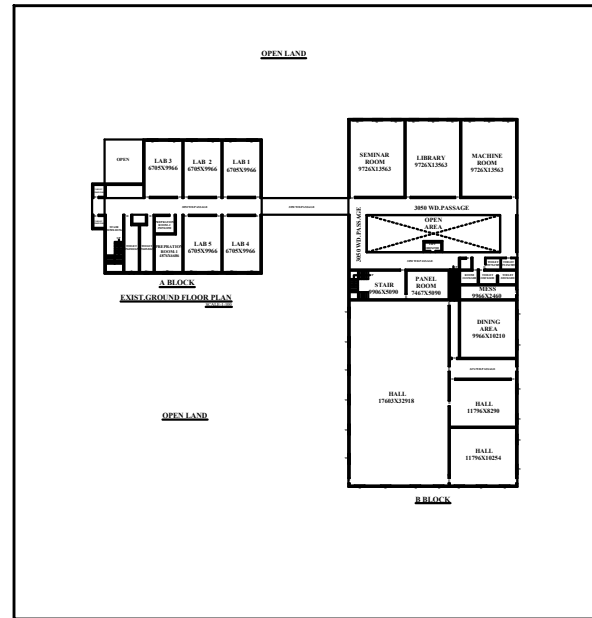
EXIST. GROUND FLOOR PLAN SCALE: 1/50
