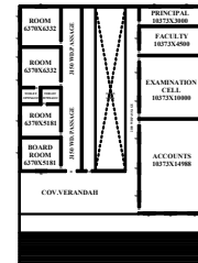
EXIST. GROUND FLOOR PLAN SCALE: 1/50
