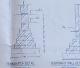
FOUNDATION DETAIL (METER SCALE) BOUNDARY WALL DETAIL (METER SCALE)
