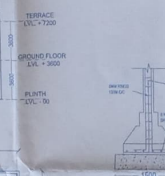
R.C.C FOUNDATION NOT TO SCALE
