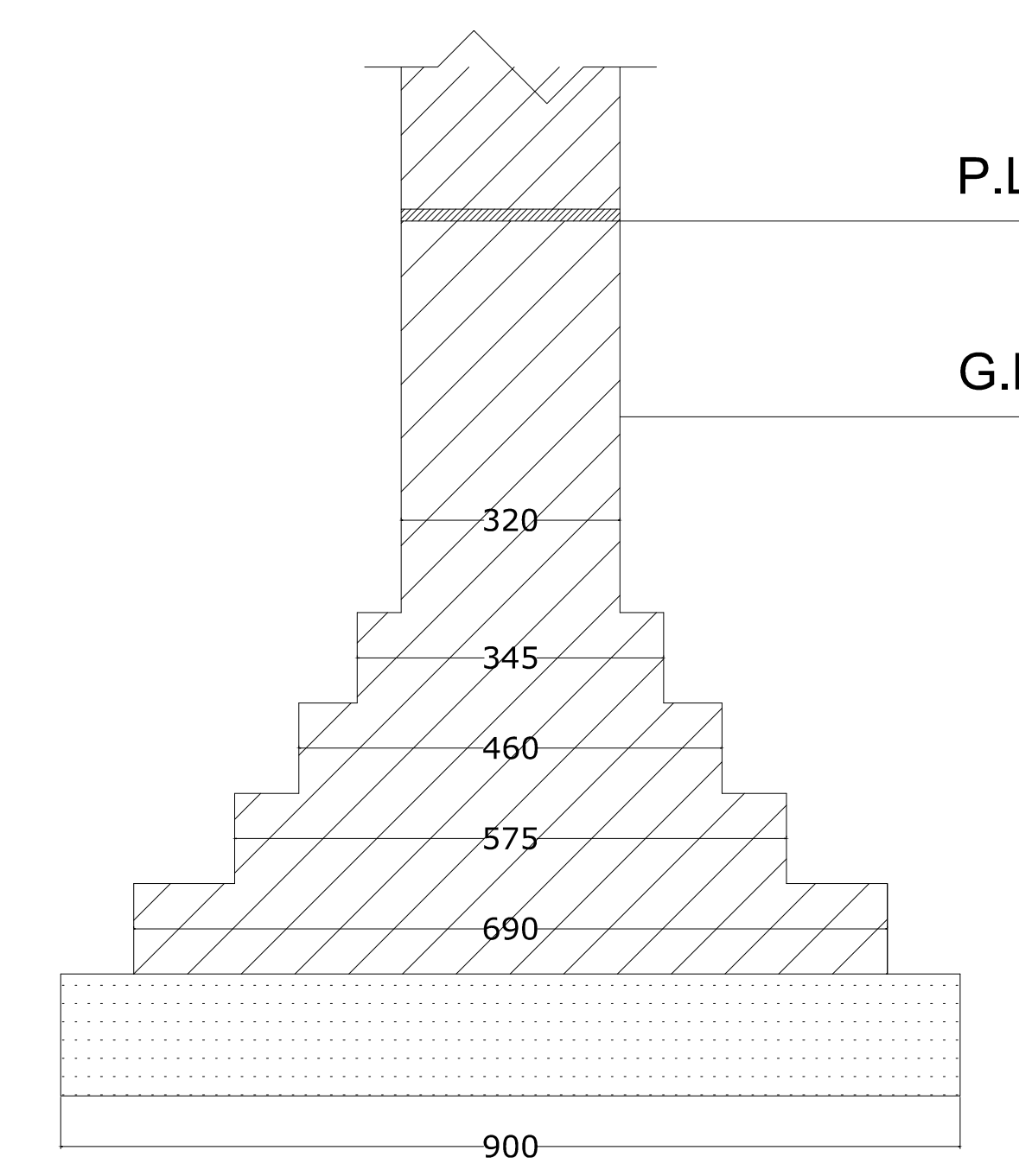
FOUNDATION DETAILS NOT TO SCALE
