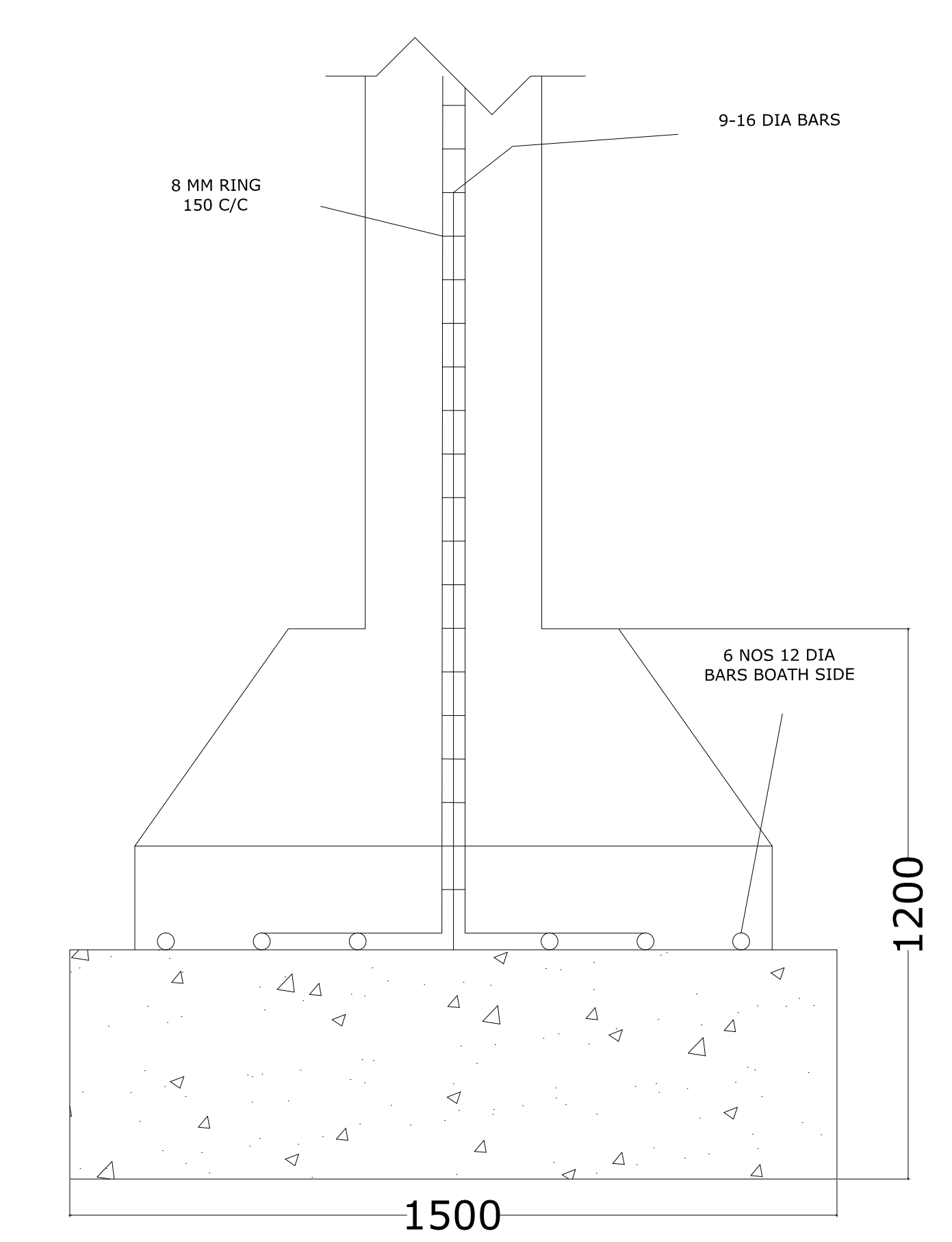
R.C.C. FOUNDATION NOT TO SCALE
