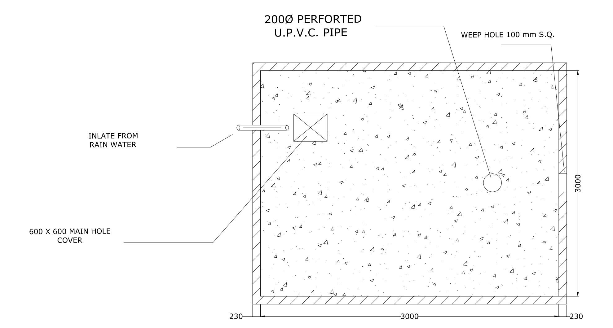
PLAN WATER RECHARGING PIT NOT TO SCALE 6.00 MT DEEP
