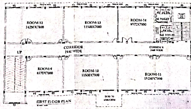
TERRACE PLAN SCALE: 1/4" = 1'-0"
