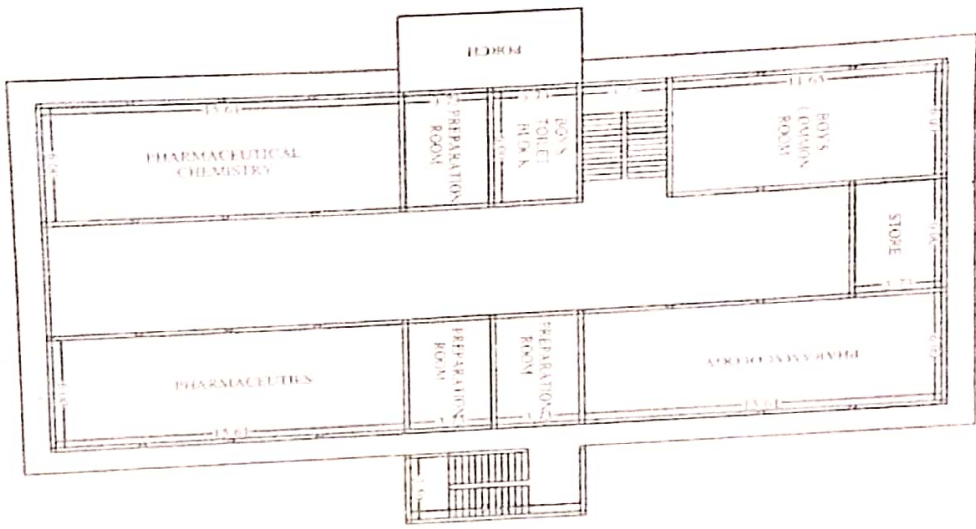
FIRST FLOOR PLAN BLOCK 101
