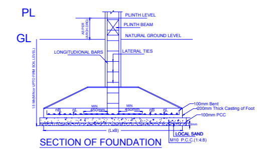
FOUNDATION DETAIL
