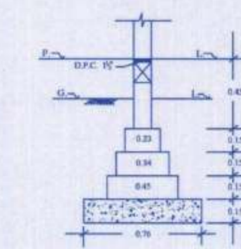
DETAIL OF BRICK FOUNDATION
