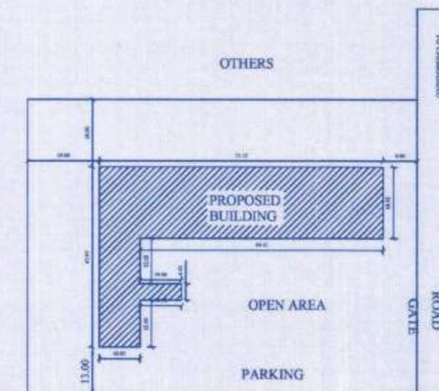
OTHERS SITE PLAN SCALE 1:1000
