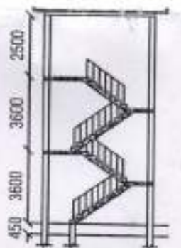
STAIR SECTION
