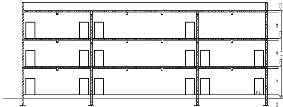
SECTION AT X-X
