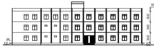
FRONT ELEVATION
