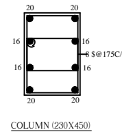
COLUMN (230X450)
