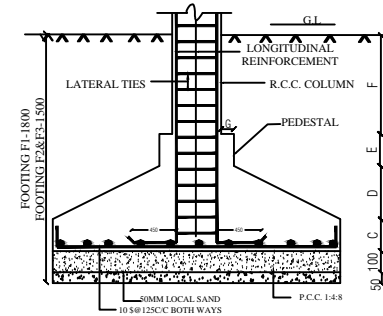
FOUNDATION DETAIL
