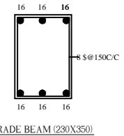
GRADE BEAM (230X350)
