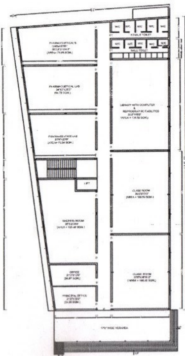
GROUND FLOOR PLAN (Sc.-1"=8'-0")
