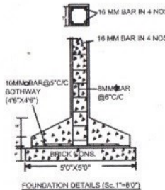
FOUNDATION DETAILS (Sc.-1"=8'-0")
