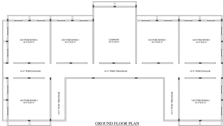
GROUND FLOOR PLAN (PART-B)
