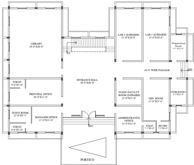
GROUND FLOOR PLAN (PART-A)
