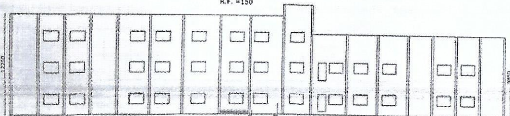
REAR ELEVATION
