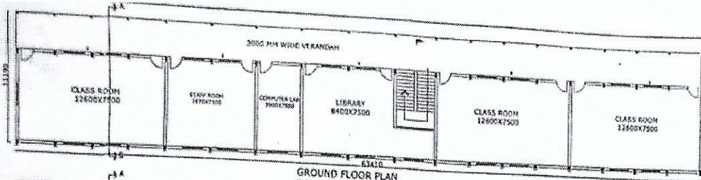
GROUND FLOOR PLAN R.F. = 150
