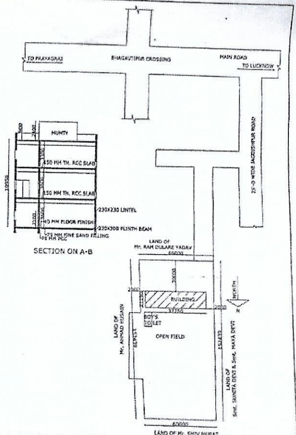
KEY & SITE PLAN (NOT TO SCALE)
