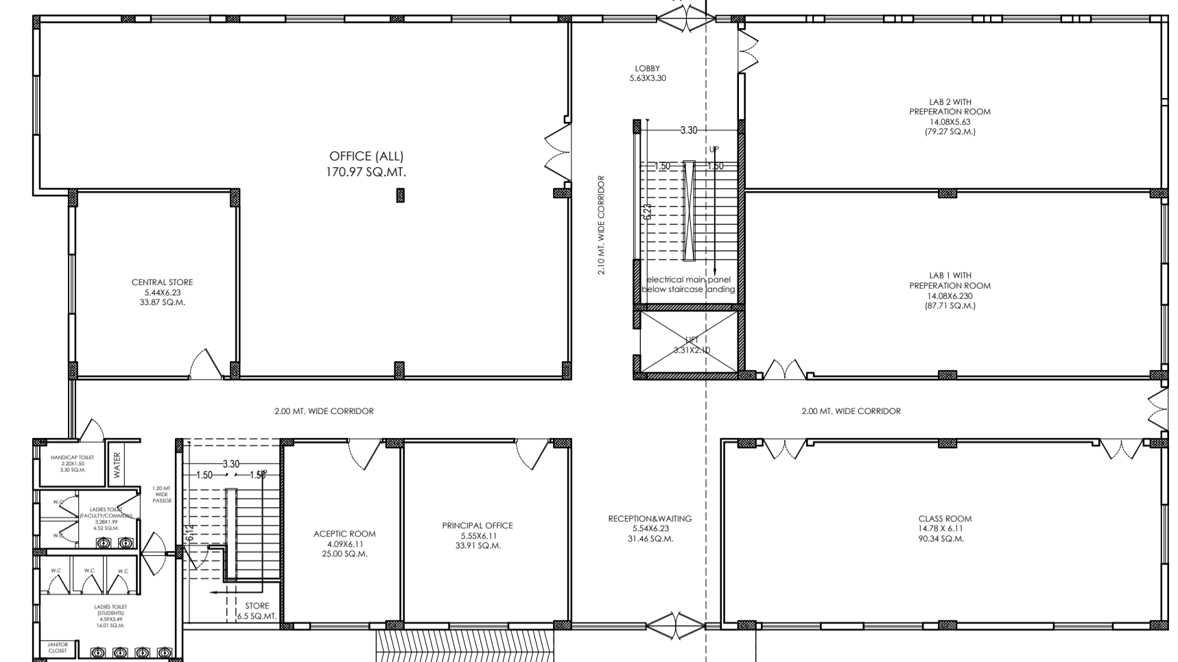
GROUND FLOOR PLAN ACADEMIC BLOCK
