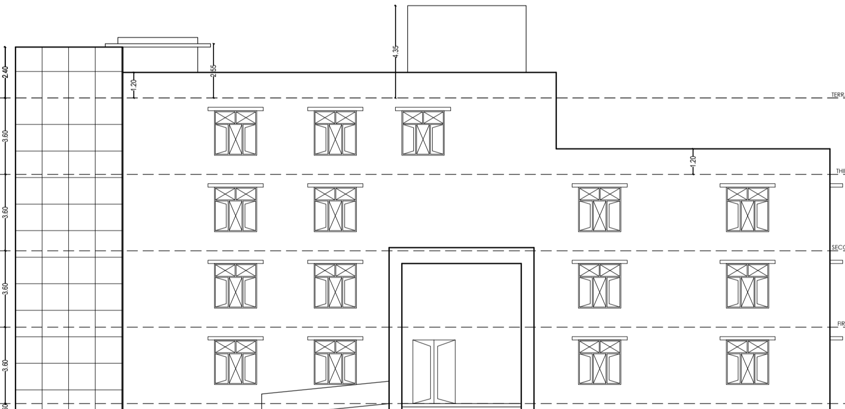
FRONT ELEVATION ACADEMIC BLOCK
