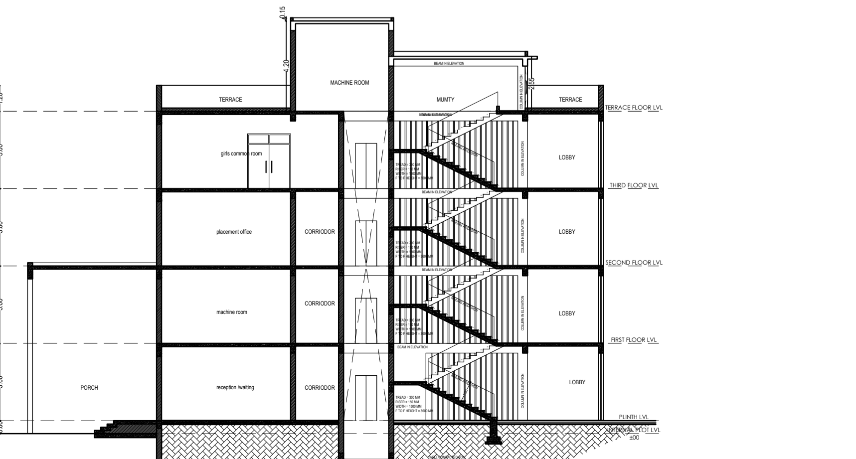
SECTION AT X-X ACADEMIC BLOCK
