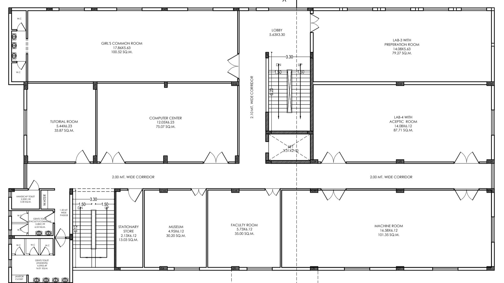
FIRST FLOOR PLAN ACADEMIC BLOCK
