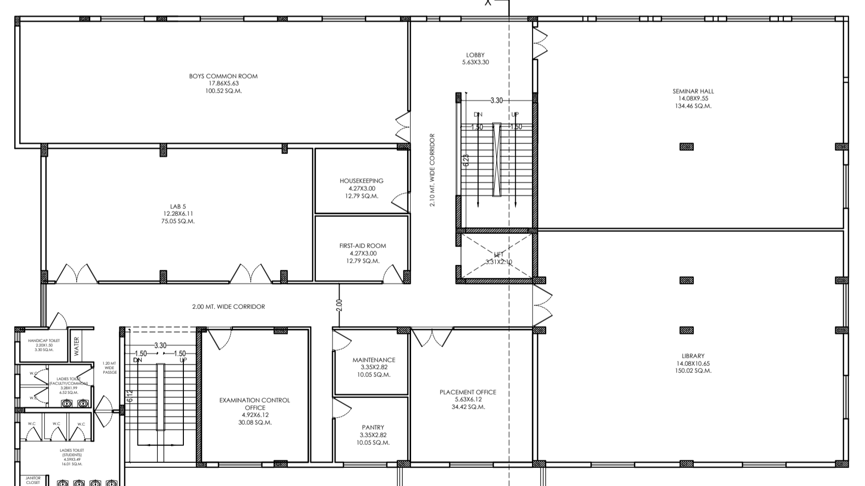
SECOND FLOOR PLAN ACADEMIC BLOCK
