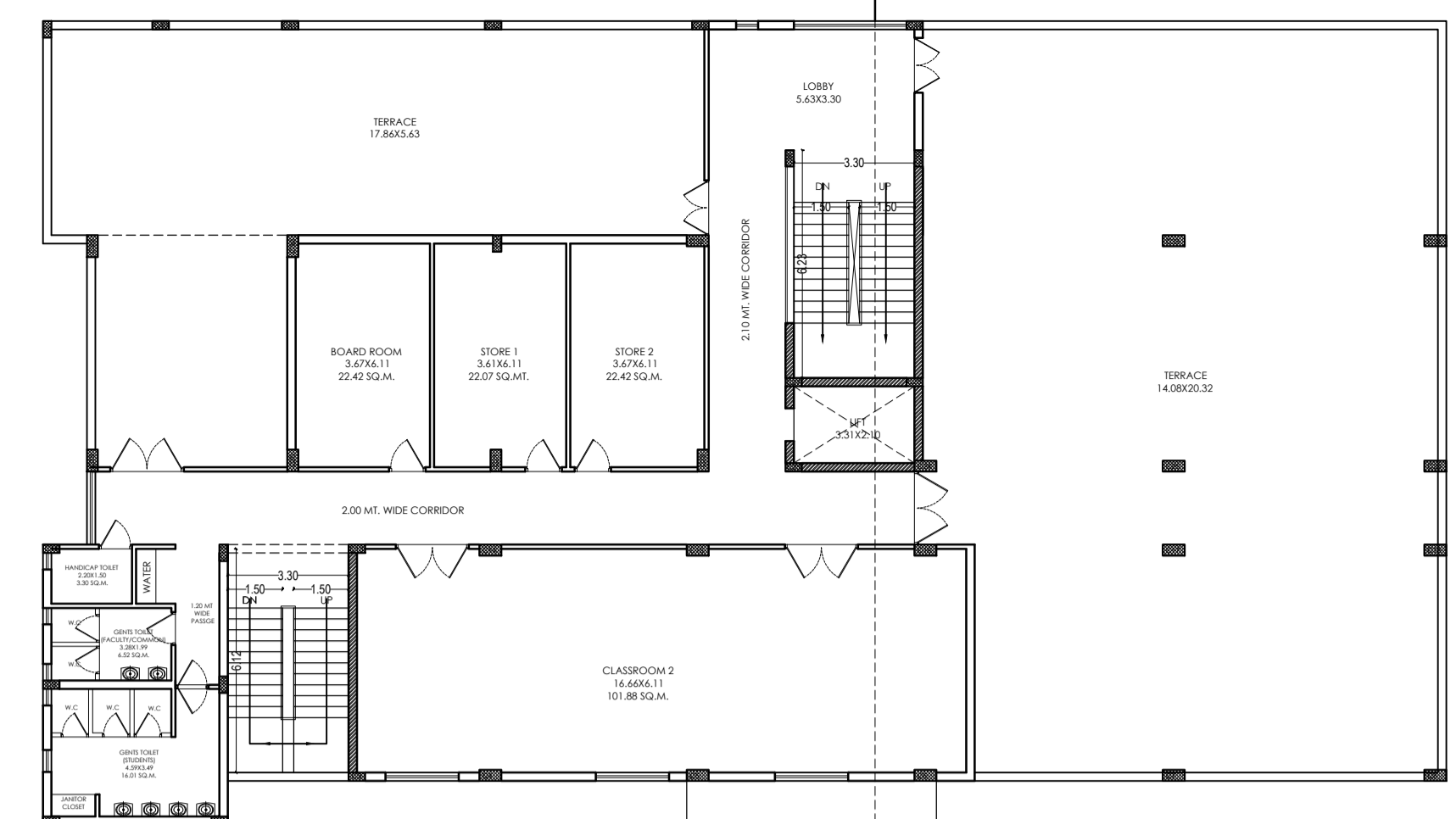
THIRD FLOOR PLAN ACADEMIC BLOCK
