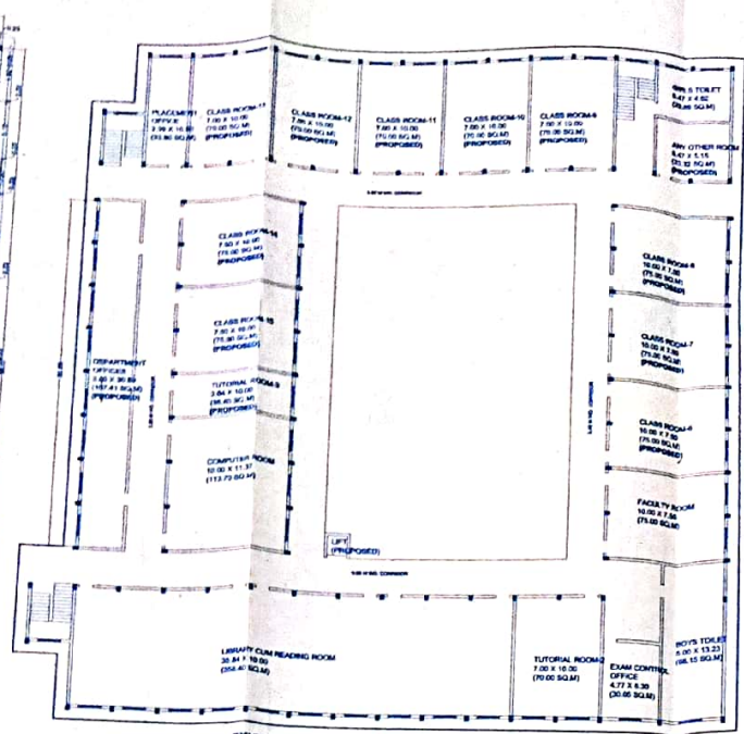
EXISTING & PROPOSED FIRST FLOOR PLAN (BLOCK-A) SCALE: 1:100
