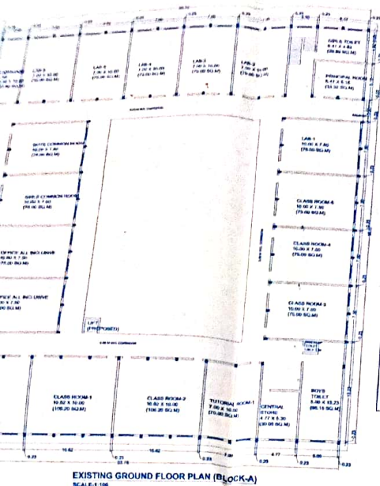
EXISTING GROUND FLOOR PLAN (BLOCK-A) SCALE: 1:100
