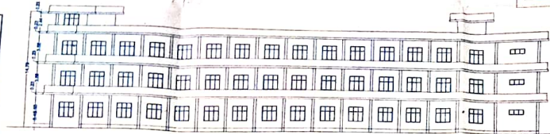
FRONT ELEVATION (BLOCK-A) SCALE: 1:100
