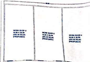
PROPOSED GROUND FLOOR PLAN (BLOCK-D) SCALE: 1:100
