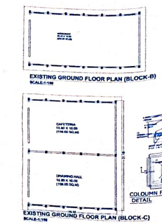
EXISTING GROUND FLOOR PLAN (BLOCK-C) SCALE: 1:100
