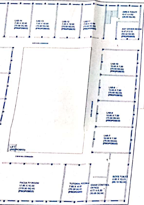
SECOND FLOOR PLAN (BLOCK-A)
