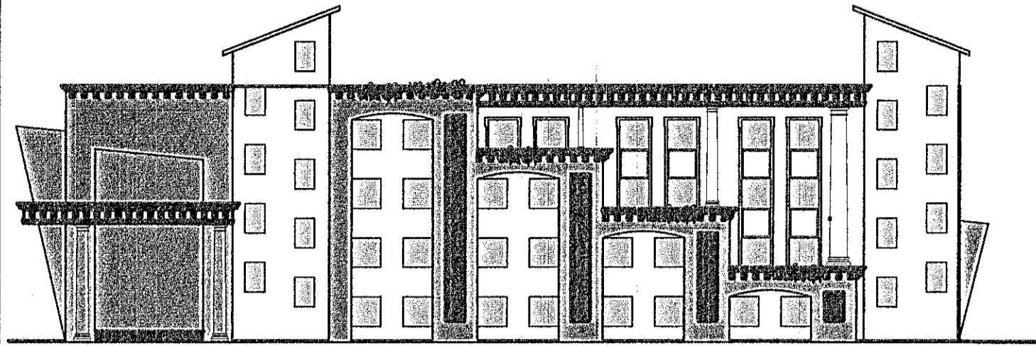
FRONT ELEVATION SCALE-1:100 BLOCK-A
