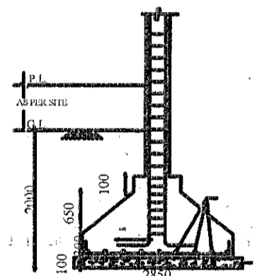
COLUMN FOOTING F2 SECTION X-X
