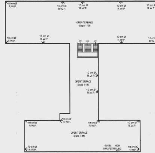
TERRACE PLAN
