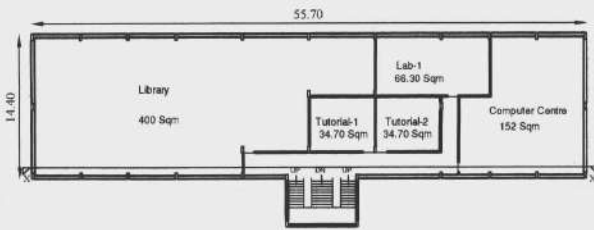
BASEMENT PLAN
